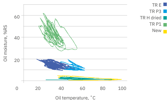
Figure 9. Hysteresis loops of %RS vs temperature in transformers with different moisture level*
