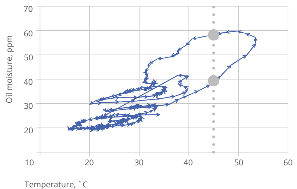
Figure 5. Moisture dynamics: hysteresis**
