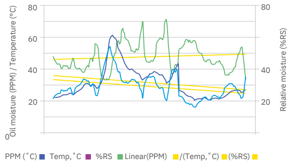
Figure 8. %RS, calculated water content and temperature with time in a 10 MVA moist aged transformer*
