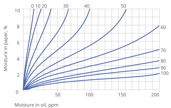
Figure 4. Moisture Equilibrium curves* (Oomen)
